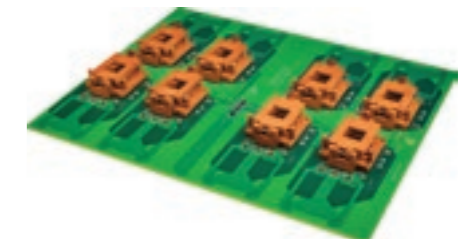
Standard test fixture for testing VLSI circuits in multisite mode using FORMULA® HF3-512 Test System
